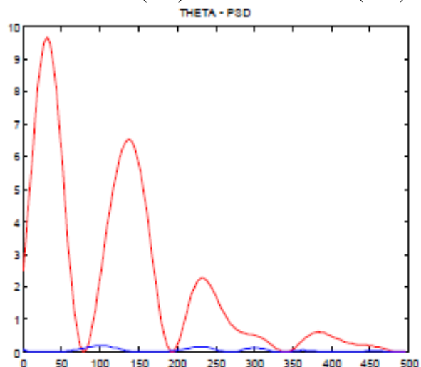
Figure 11: Power spectrum density of theta wave of normal person (red) and alcoholic person (blue)
