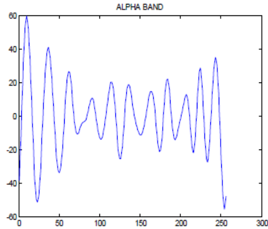
Figure 4: Alpha Band of EEG Wave Decomposed Using Stationary Wavelet Transform
