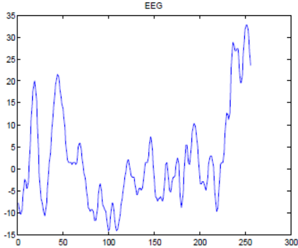
Figure 1: EEG Wave
