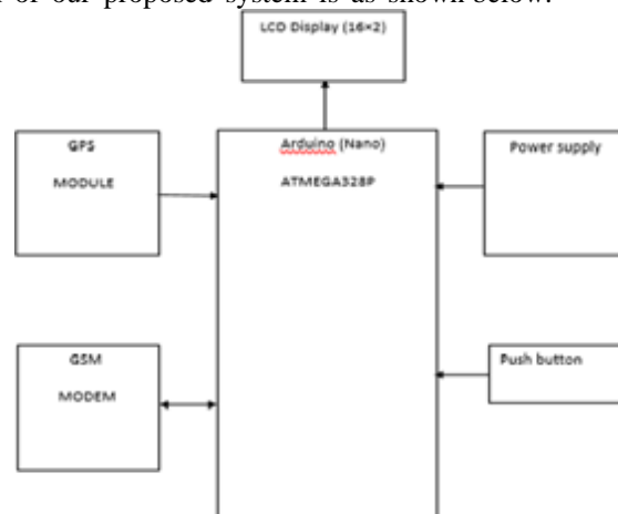
Figure 1: Block Diagram of Women Security System
